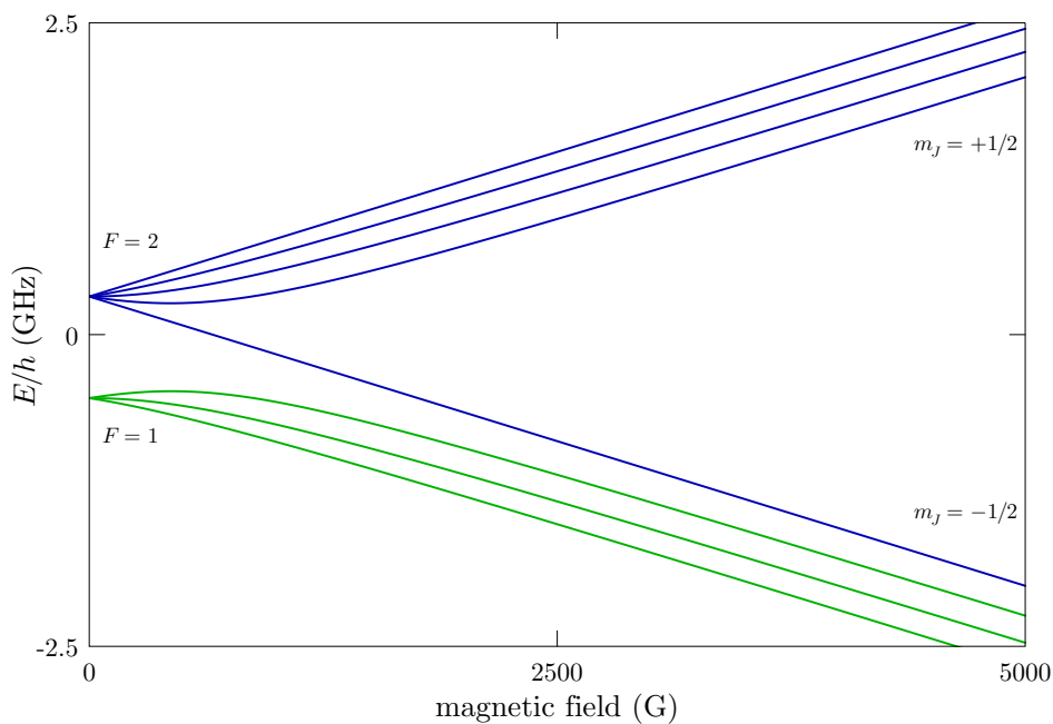
Figure 5: Rubidium 87 5^2P_{1/2} ( D_1 excited) level hyperfine structure in an external magnetic field. The levels are grouped according to the value of F in the low-field (anomalous Zeeman) regime and m_j in the strong-field (hyperfine Paschen-Back) regime.
