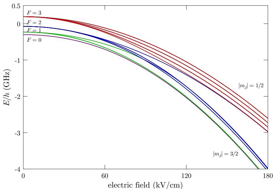
Figure 7: Rubidium 87 5^2P_{3/2} ( D_2 excited) level hyperfine structure in a constant, external electric field. The levels are grouped according to the value of F in the low-field (anomalous Zeeman) regime and |m_J| in the strong-field ("electric" hyperfine Paschen-Back) regime. Levels with the same values of F and |m_F| (for a weak field) are degenerate.
