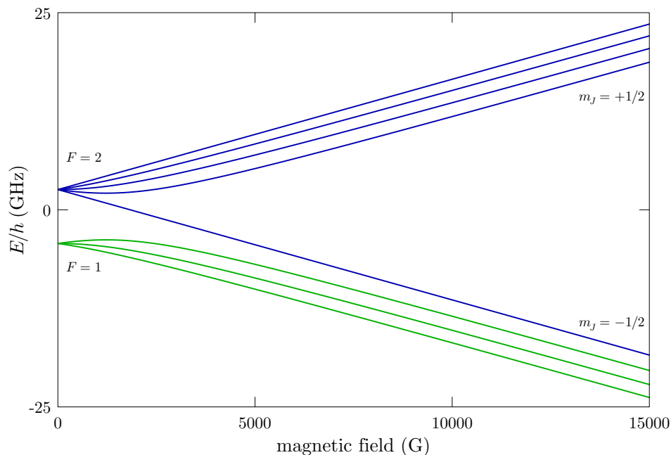
Figure 4: Rubidium 87 5^2S_{1/2} (ground) level hyperfine structure in an external magnetic field. The levels are grouped according to the value of F in the low-field (anomalous Zeeman) regime and m_j in the strong-field (hyperfine Paschen-Back) regime.
