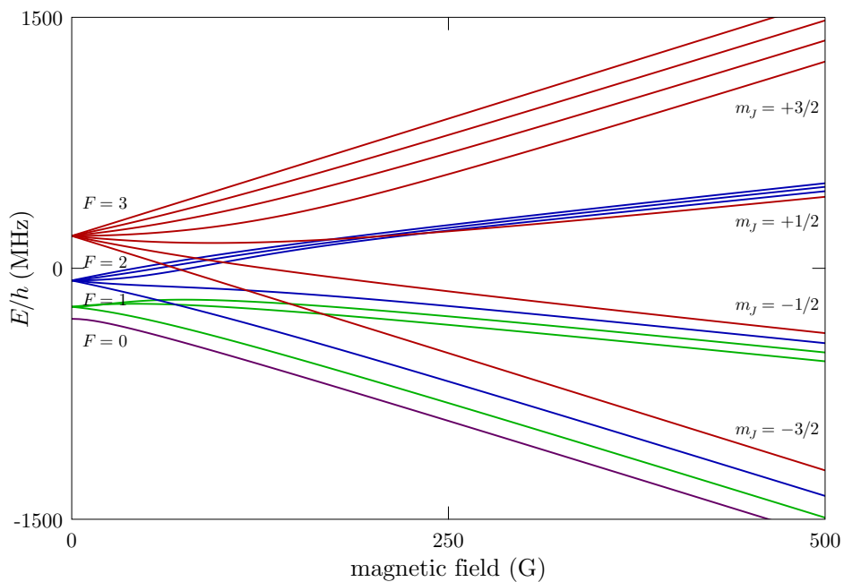
Figure 6: Rubidium 87 5^2P_{3/2} ( D_2 excited) level hyperfine structure in an external magnetic field. The levels are grouped according to the value of F in the low-field (anomalous Zeeman) regime and m_J in the strong-field (hyperfine Paschen-Back) regime.
