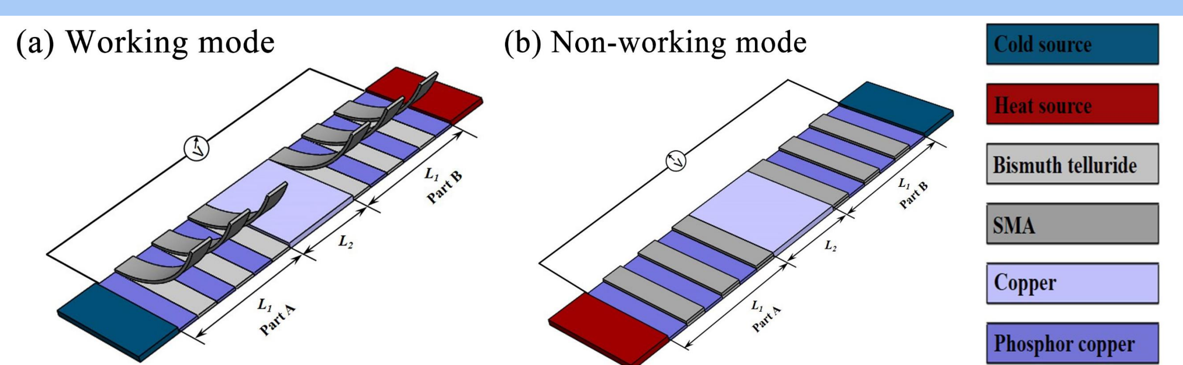
Fig. 2 Schematic drawing for experimental demonstration
