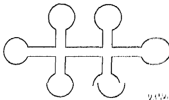
Fig. 2. The bridge-shaped sample, furnished with large areas for making low-ohmic contacts. large areas at the ends have the task to provide low-ohmic contacts. Furthermore, when making these contacts a heat treatment is often necessary which in this case can be done without heating that part of the sample which is under measurement.
