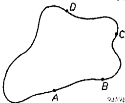
Fig. 3. A sample of arbitrary shape with four small contacts at arbitrary places along the circumference which, according to this paper, can be used to measure the specific resistivity and the Hall effect.
