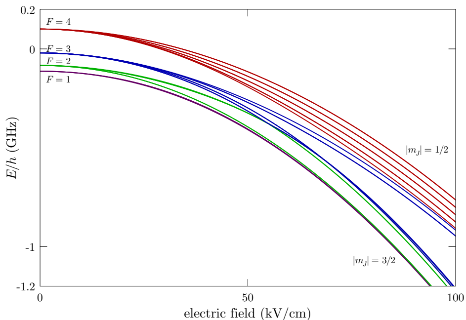
Figure 7: Rubidium 85 5^2P_{3/2} ( D_2 excited) level hyperfine structure in a constant, external electric field. The levels are grouped according to the value of F in the low-field (anomalous Zeeman) regime and |m_J| in the strong-field ("electric" hyperfine Paschen-Back) regime. Levels with the same values of F and |m_F| (for a weak field) are degenerate.
