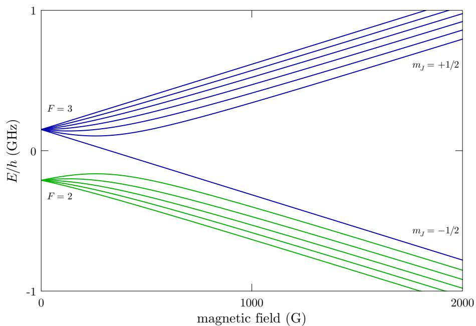
Figure 5: Rubidium 85 5^2P_{1/2} (D 1 excited) level hyperfine structure in an external magnetic field. The levels are grouped according to the value of F in the low-field (anomalous Zeeman) regime and m_j in the strong-field (hyperfine Paschen-Back) regime.
