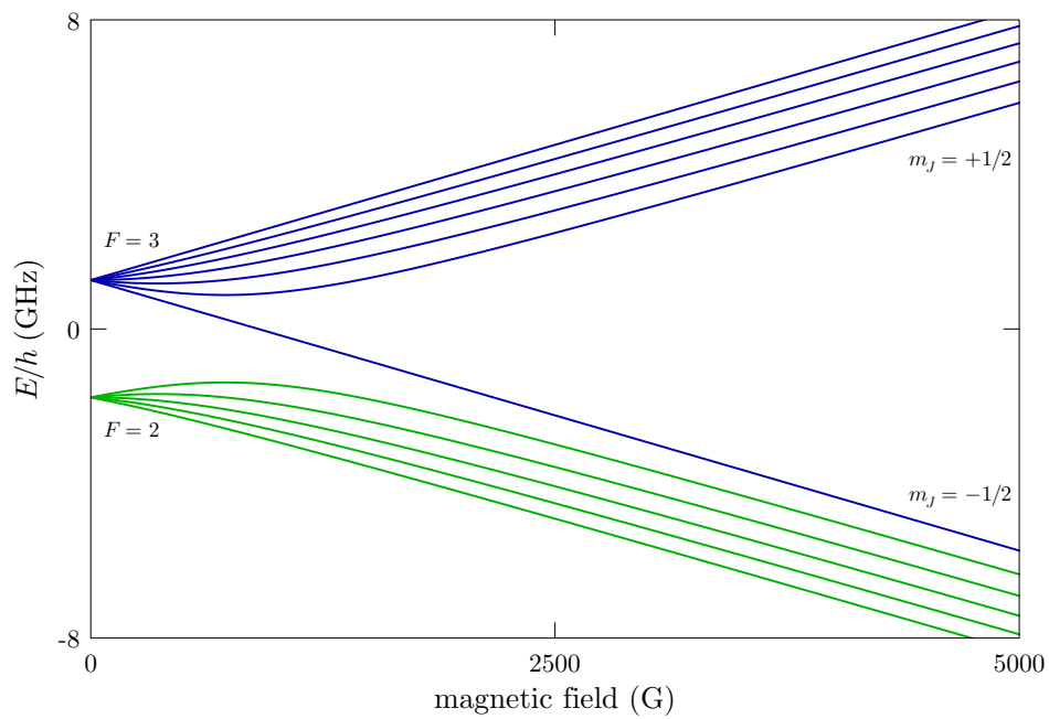
Figure 4: Rubidium 85 5^2S_{1/2} (ground) level hyperfine structure in an external magnetic field. The levels are grouped according to the value of F in the low-field (anomalous Zeeman) regime and m_j in the strong-field (hyperfine Paschen-Back) regime.
