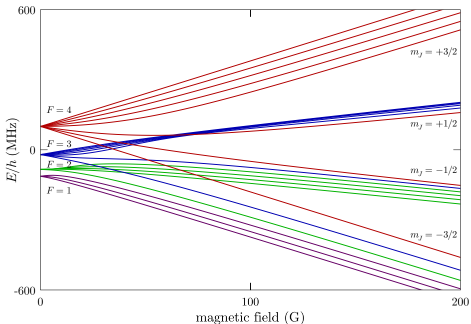
Figure 6: Rubidium 85 5^2P_{3/2} ( D_2 excited) level hyperfine structure in an external magnetic field. The levels are grouped according to the value of F in the low-field (anomalous Zeeman) regime and m_J in the strong-field (hyperfine Paschen-Back) regime.
