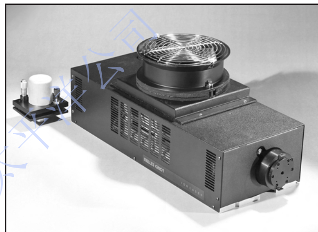
Prism-tunable-ion laser
