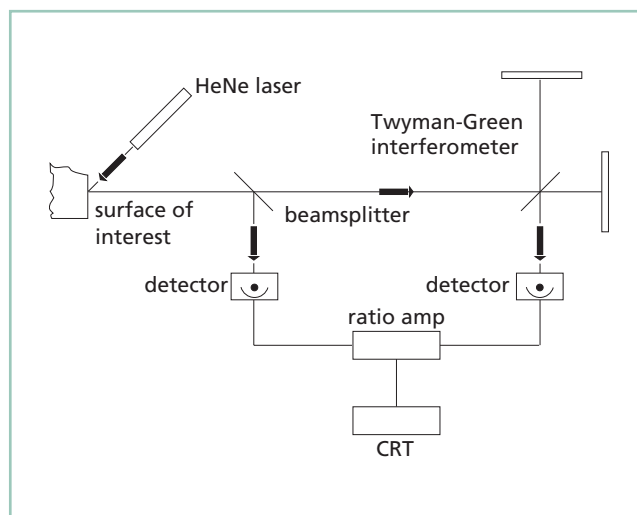
Figure 36.32 Interferometric measurement
