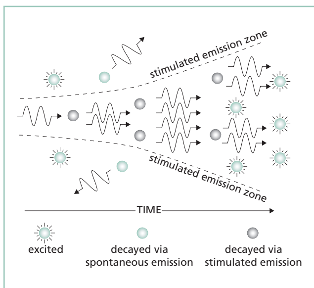
Figure 36.3 Amplification by stimulated emission
