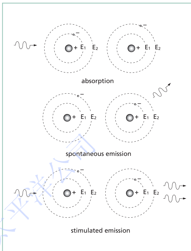
Figure 36.2 Spontaneous and stimulated emission
