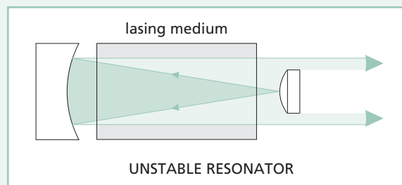
Unstable Resonator Design
