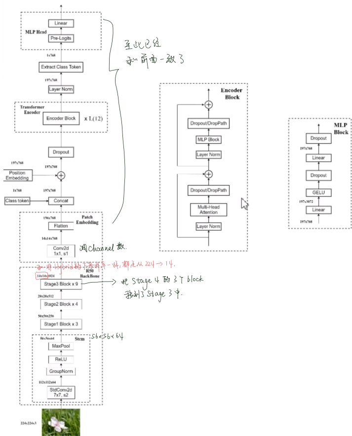
R50+ViT-B/16 hybrid model
